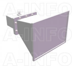
LB-650-10-C-7/16FSPO Standard Gain Horn Antenna 1.12-1.7GHz 10dB Gain 7/16(DIN) Female
